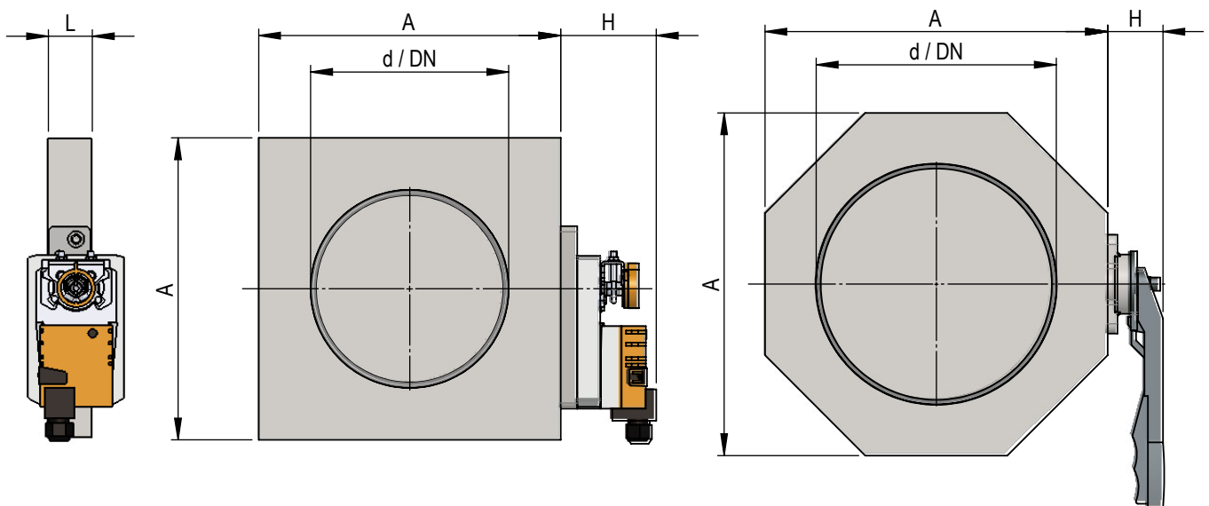
Design 1 DN50 - DN200
